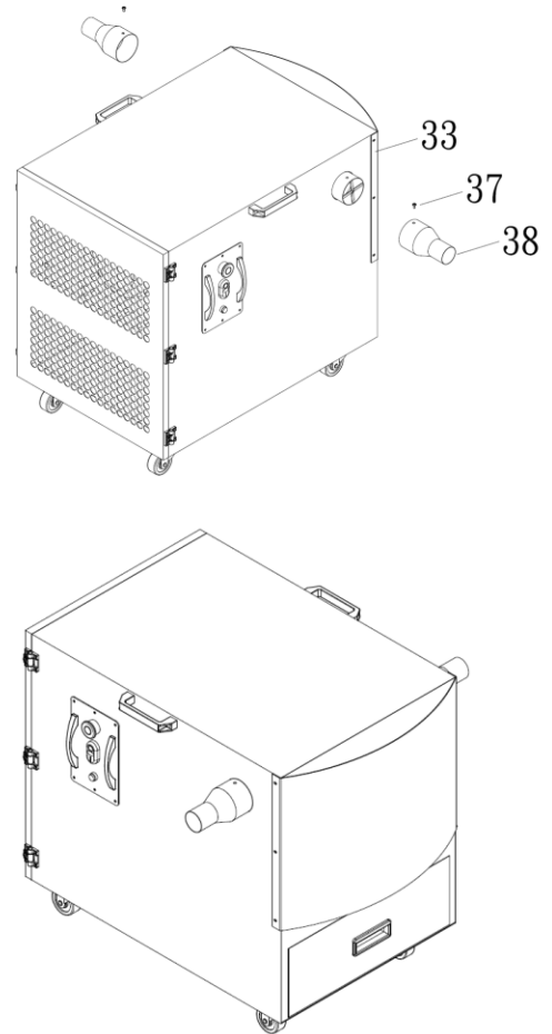
Figure 8-2: Hose Adaptor Installation
