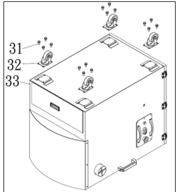
Figure 8-1: Caster Installation
