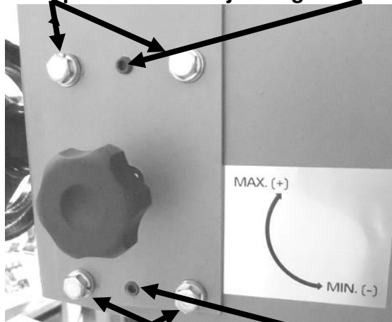
Clamping bolts A Jack bolt B
