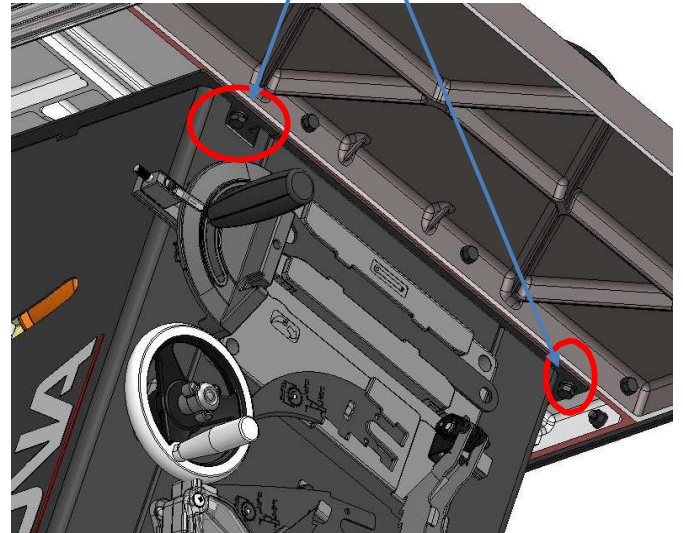
Fig. H: Aligning Table (view from under table top)
