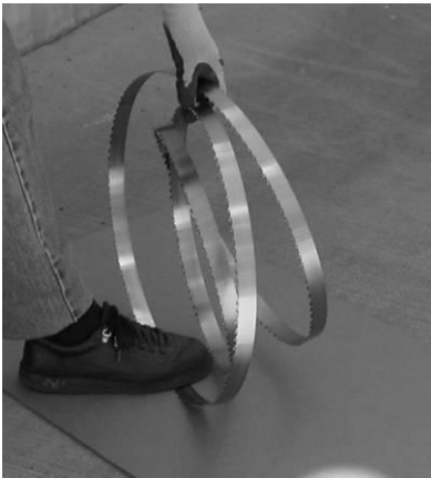
Blade coiling
